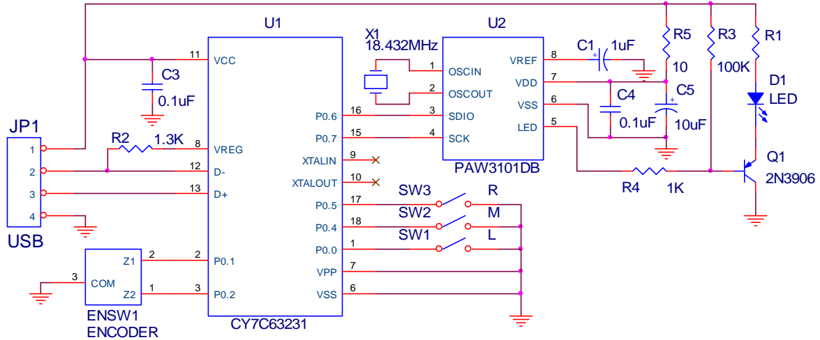
Figure 11. 5V Application Circuit with External LED Control
