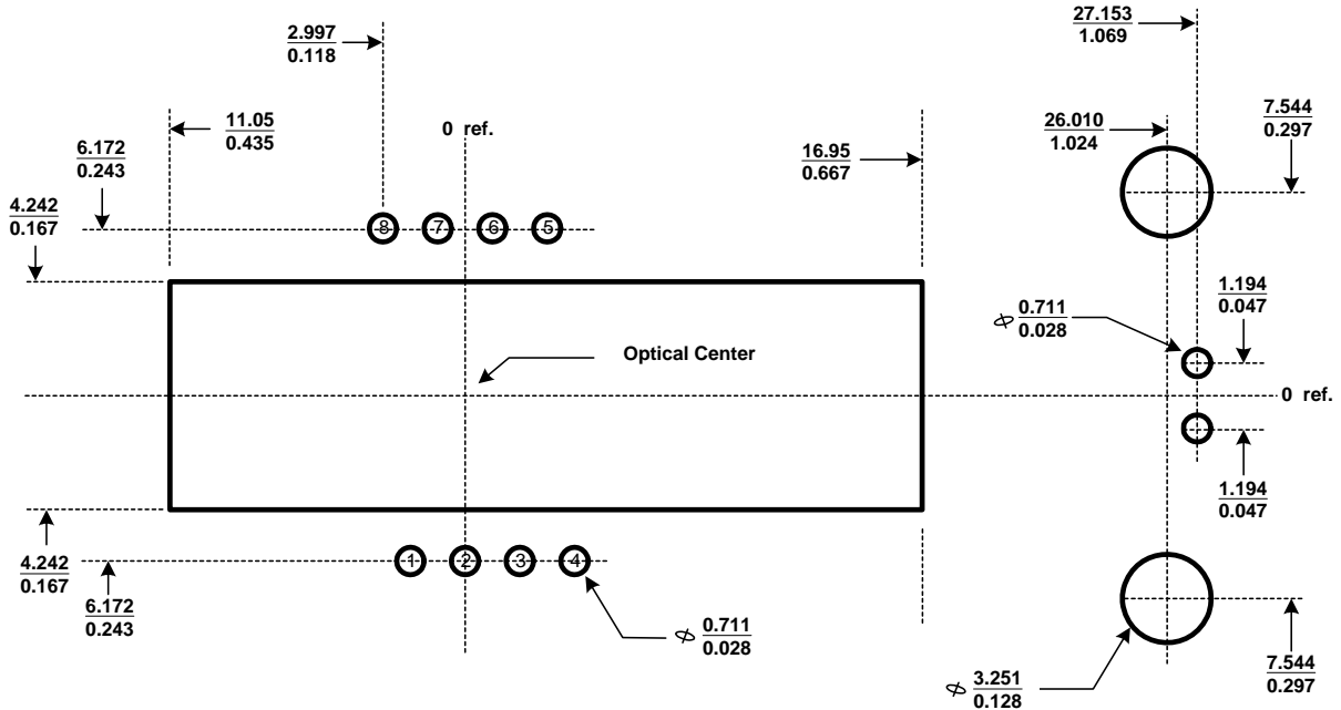
Figure 15. Recommended PCB Mechanical Cutouts and Spacing
